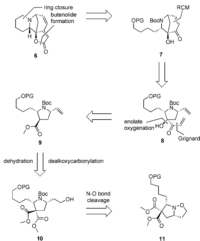
Scheme 2. A retrosynthesis for (–)-allosecurinine. RCM = ring-closing metathesis.
